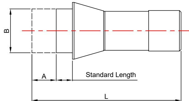
Standard Model + Custom A/L Dimension
